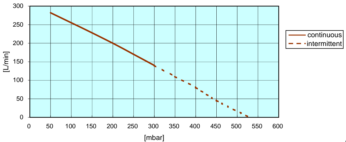
HP 200 Q-H Performance Curves
