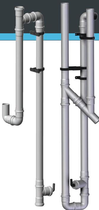
Mamut-pumpe u postrojenju STABI-S
